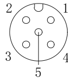
Pin Assignment Front View M12 male A-Coding 5PIN
