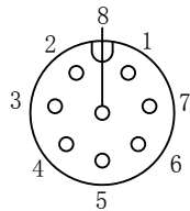
Pin Assignment Front View MALE
