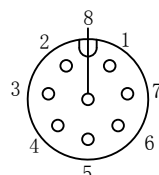
Pin Assignment Front View MALE
