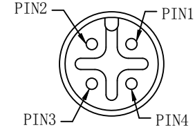
Pin Assignment Front View MALE
