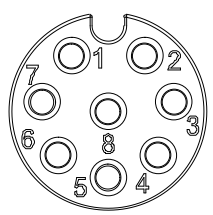
Pin Assignment Front View M12 female A-Coding 8PIN
