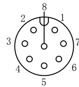
Pin Assignment Front View MALE
