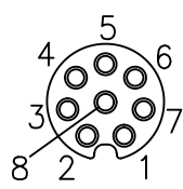
Pin Assignment Front View M8 female A-Coding 8PIN
