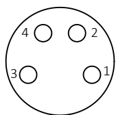
Pin Assignment Front View M8 female A-Coding 4PIN
